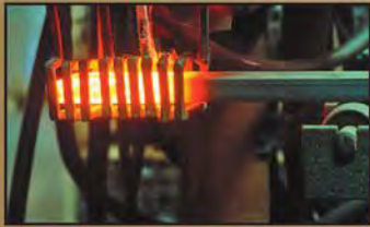
The raw steel is heated to 1200°C and cut into suitable lengths depending on what type of axe is to be made.
